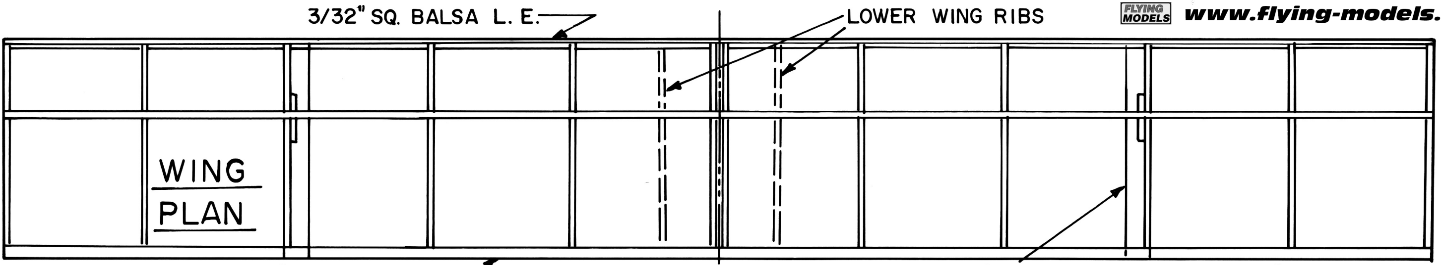
TOP VIEW
